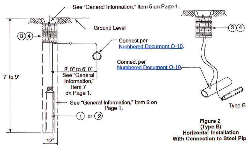
Figure 1 (Type A) Typical Vertical Installation With Connection to Steel Pipe
