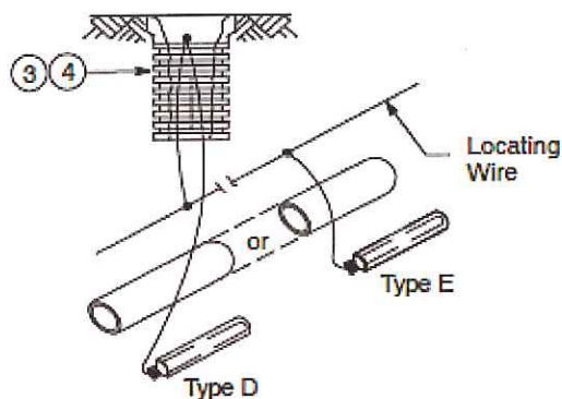
Figure 3 (Type D and E) Horizontal Installation With Connection to Plastic Pipe
