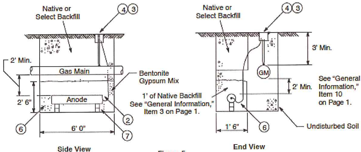
Figure 5 Horizontal Installation of Bare Galvanic Anodes for Mains 3' Deep or Deeper
