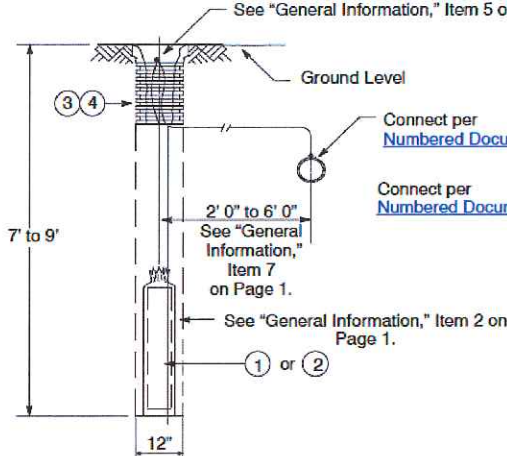
Figure 1 (Type A) Typical Vertical Installation With Connection to Steel Pipe
