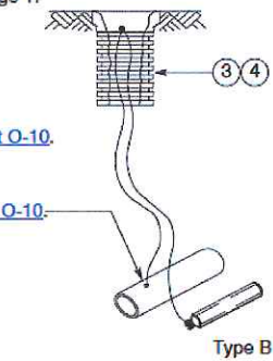
Figure 2 (Type B) Horizontal Installation With Connection to Steel Pipe
