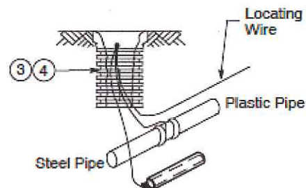
Figure 4 (Type F) Horizontal Installation With Connector to Plastic-to-Steel Transition
